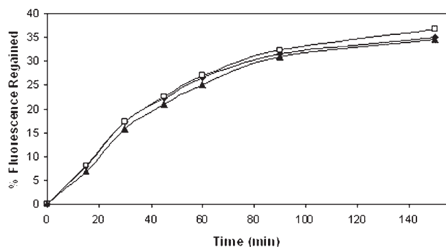
Figure 5. Percentage fluorescence intensity regained upon reaction of Z-Gly-Gly-Leu-ACA-Gly 6 -PEGA 1900 with Subtilisin Carlsberg versus time. Where □ is 0–50 µm from the bead edge to 50 µm inside the bead, ▲ is 50–100 µm and ● is 100 µm—centre of the bead. The bead diameter is 300 µm.
