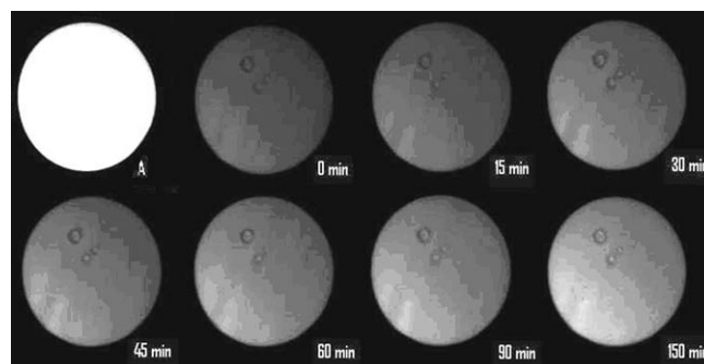
Figure 4. Two photon cross section images of Z-Gly-Gly-Leu-ACA-Gly 6 -PEGA 1900 beads, A is an uncapped amino coumarin bead. The other images are the same bead at different times of reaction with Subtilisin Carlsberg at 20 °C.
