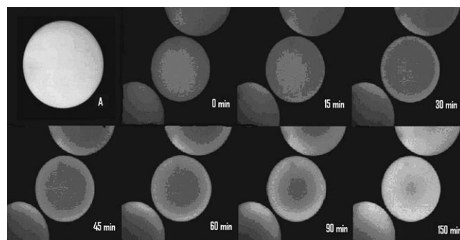
Figure 2. Two-photon cross-section images of Bz-Arg-ACA-Gly 6 -PEGA 1900 beads, A is an uncapped amino coumarin bead. The other images are the same bead at different times of reaction with acetylated trypsin at 20 °C.
