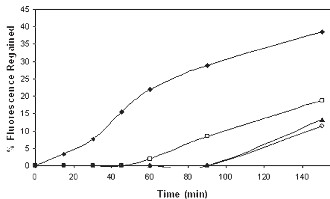
Figure 3. Percentage fluorescence intensity regained upon reaction of Bz-Arg-ACA-Gly 6 -PEGA 1900 with acetylated trypsin versus time. Each plot represents different zones within a single bead where, ◆ is 0–53 μm from the bead edge to 53 μm inside the bead, □ is 53–105 μm, ▲ is 105–158 μm and ○ is 158 μm–centre of the bead. The bead diameter was 350 μm.
