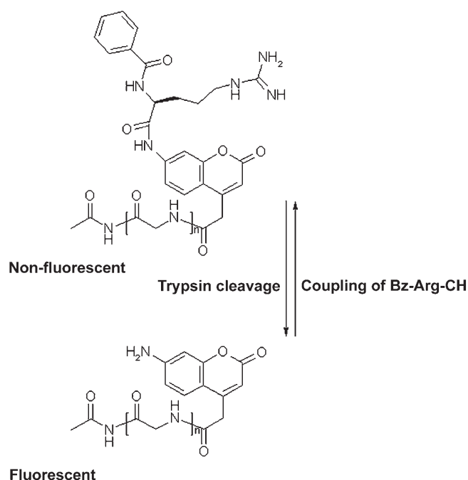
Figure 1. Schematic of coupling and enzymatic reaction processes on PEGA 1900 beads. Bz-Arg-OH is replaced with Z-Gly-Gly-Leu-OH for subtilisin reaction.
